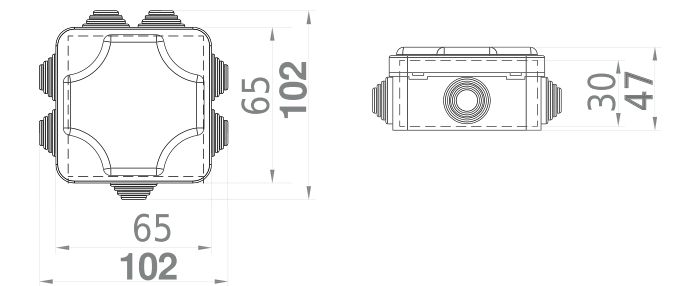
Krabice SolidBOX IP55 / Sealed box IP55 - Objč. / Item 68012
