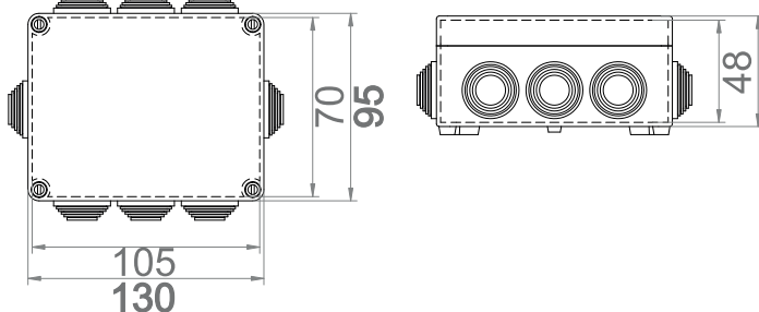
Krabice SolidBOX IP55 / Sealed box IP55 - Objč. / Item 68032
