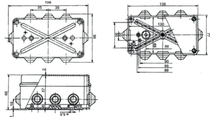
Krabice SolidBOX IP55 / Sealed box IP55 - Objč. / Item 68052
