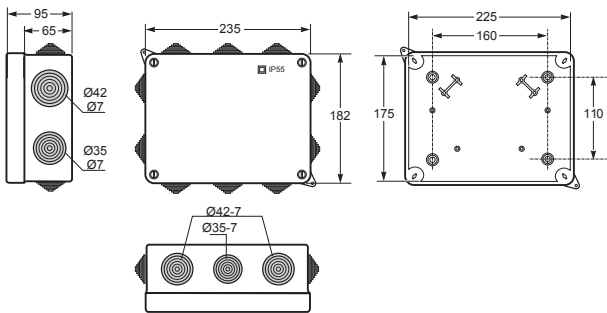
Krabice AcquaBOX IP55 / Box with cones IP55 - Obj.č. / Item 3014
